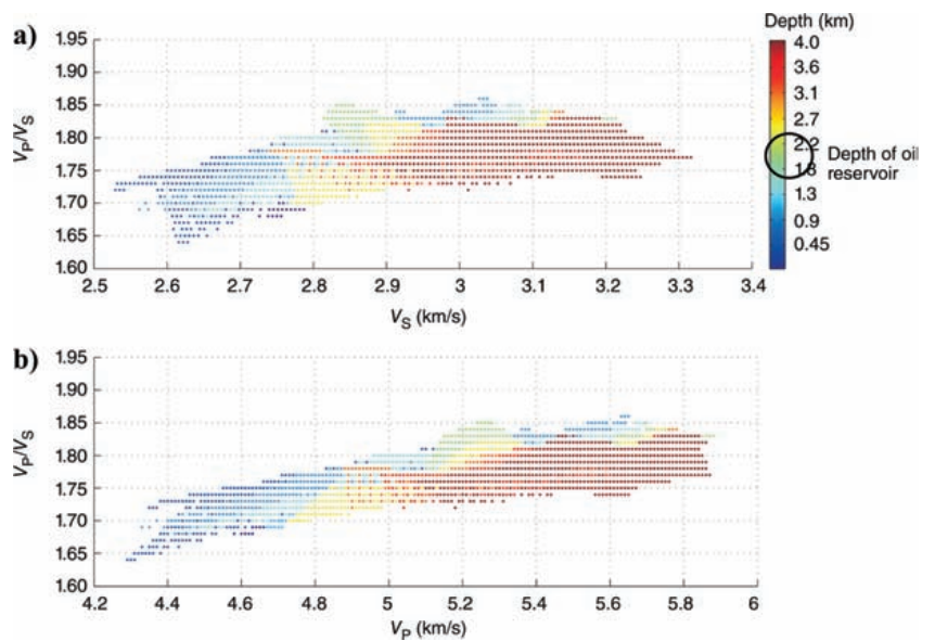
Figure 24. Relation between V_P/V_S and (a) V_S and (b) V_P for the oil-producing area at various depths.
