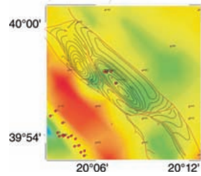
Figure 17. Correlation between preexisting data interpretation and PST results at 3.5-km depth (from mean sea level), focusing on the Delvina gas-production area. Contours depict depth to the limestone. Damping is 3.5 km; grid spacing is 1000 m.
