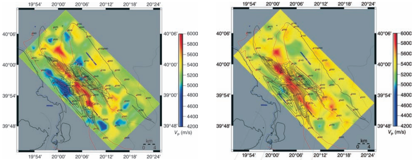
Figure 16. Correlation between preexisting data interpretation and PST results at 2-km depth (from mean sea level). Contours depict known depths to the limestone. Damping is 2 km; grid spacing is 1000 m.
