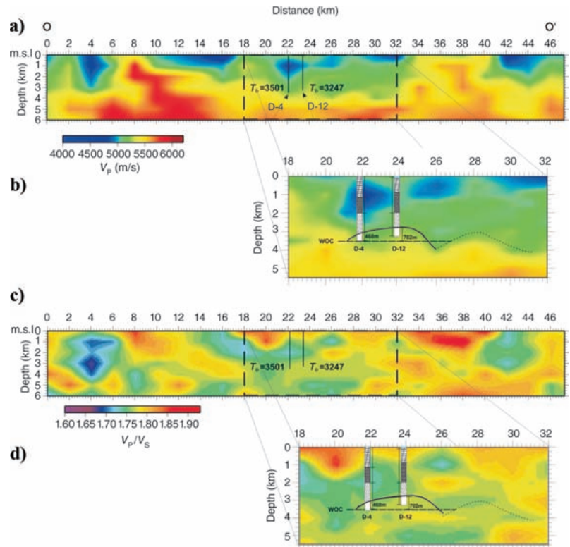
Figure 19. (a) The V_P cross sections along line OO'. (b) Comparison with wells D-4 and D-12. (c) The V_P/V_S cross sections along line OO'. (d) Comparison with wells D-4 and D-12. Dashed line labeled WOC is the water-oil contact. The dotted line presents a possible second anticline.
