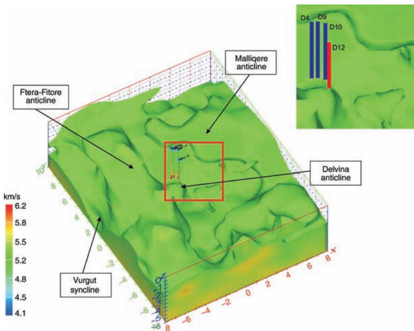
Figure 18. A 3D view of the Delvina anticline structure and surrounding structures based on PST results ( V_p > 5.24 ). Upper right is a close-up view of a section of the structure.
