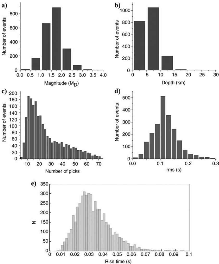
Figure 5. Histogram of (a) microearthquake magnitudes, (b) hypocenter depths, (c) number of peaks, (d) rms, and (e) rise times.
